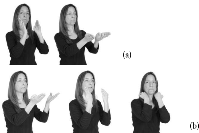
Figure 4: Two forms of the ASL verb CONVINCING: (a) CONVINCING-him and (b) CONVINCING-me.
