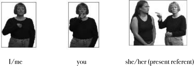
Figure 2. Deictic pointing signs in ASL.
